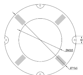
Holder for Lifebuoy Ring & Horseshoe
