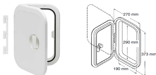
Removable Hinge "2 In 1" Hatch Cover
