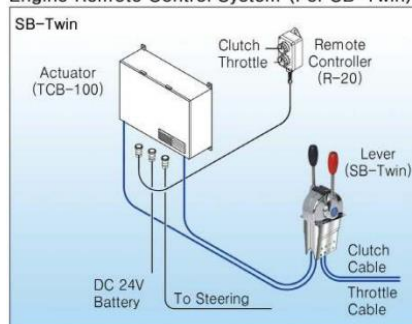
Engine Remote Control System (For SB-Twin)
