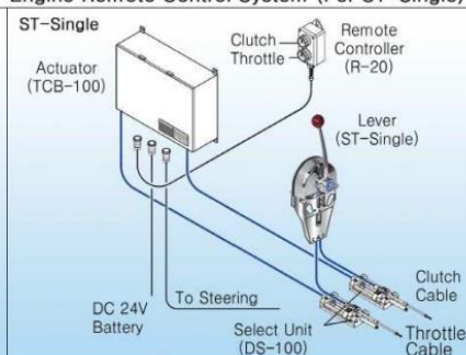
Engine Remote Control System (For ST-Single)
