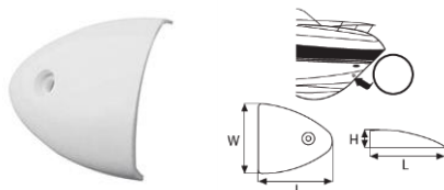
Ventilation Clam Shell Cover, white
